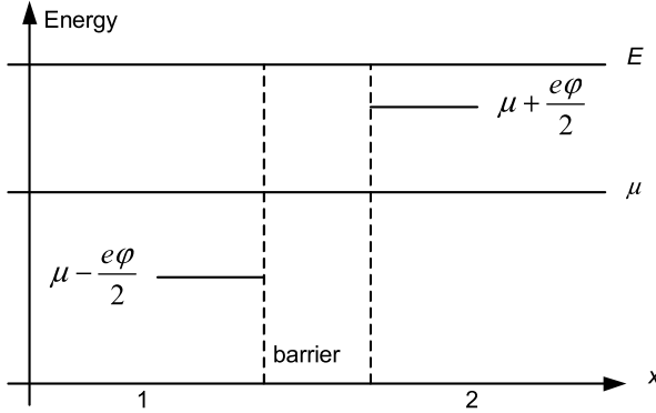
Fig. 12.7. Tunneling sketch
