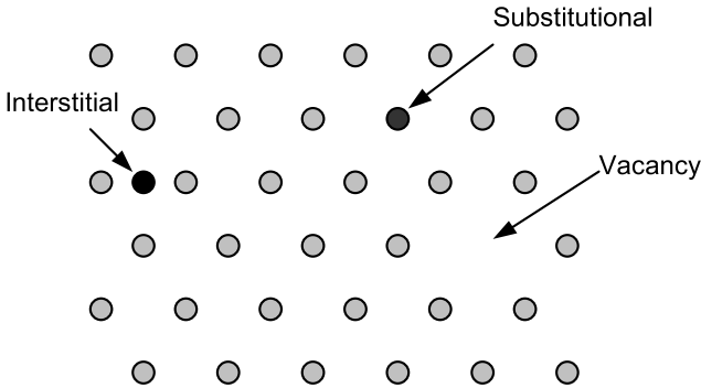
Fig. 11.1. Point defects
